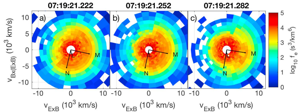
Figure 4. Evolution of phase space density of perpendicular electron distribution observed by MMS3 around the time of the largest amplitude v_{e,M} on the right-hand side of the current sheet. The horizontal axis is the local \mathbf{E} \times \mathbf{B} direction, while the vertical axis is the local \mathbf{B} \times (\mathbf{E} \times \mathbf{B}) direction. For reference, we have overplotted arrows marking the fixed LMN coordinate system. Further away from the center of the current sheet, the higher energy population ( \sim 5,000 km/s) covers a smaller azimuthal interval. This feature is consistent with the finite gyroradius effect observed both in simulations and observations of magnetic reconnection.
