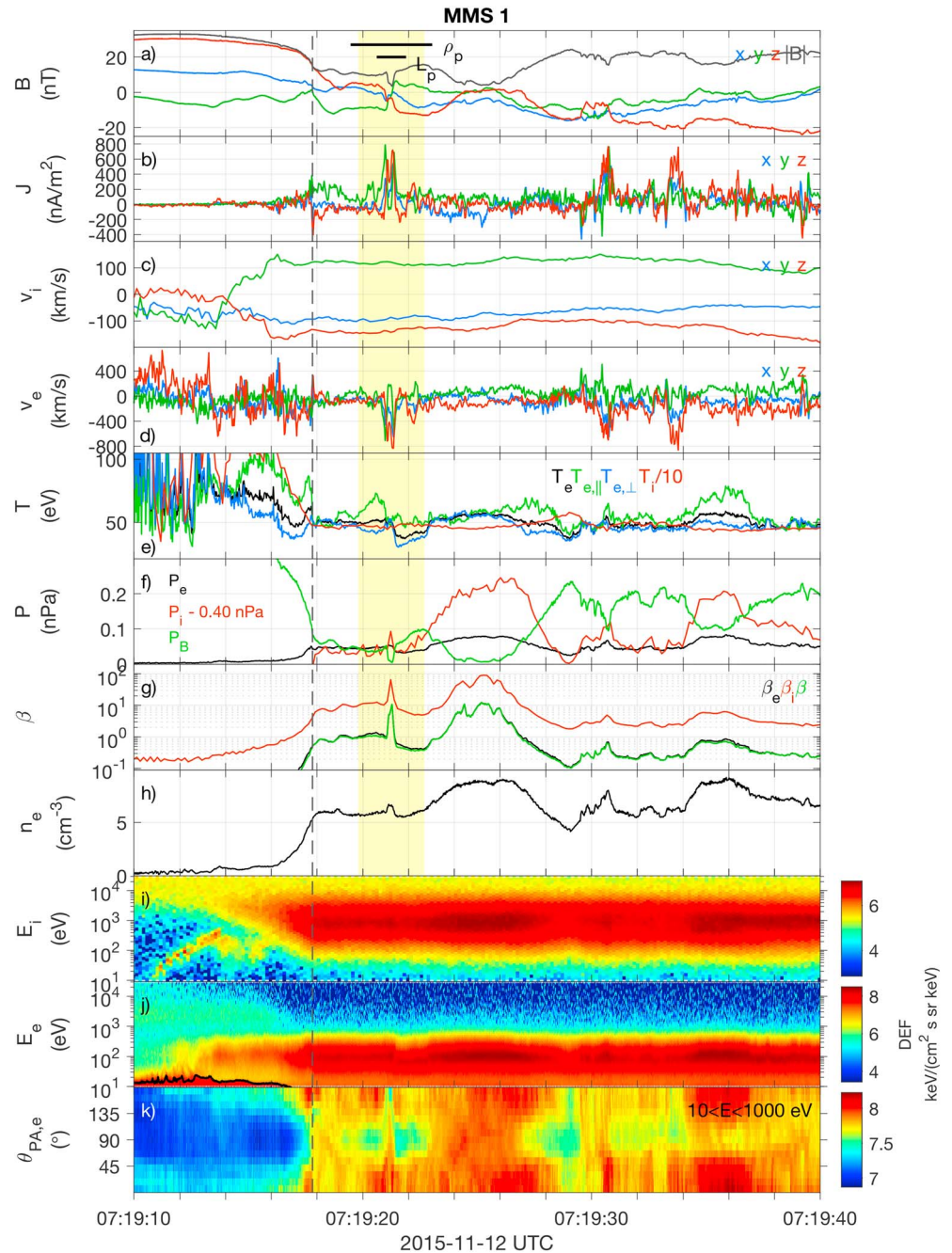
Figure 1. Overview of magnetopause crossing as seen by MMS1. All vectors are given in Geocentric Solar Ecliptic coordinates. The black-dashed line marks the magnetosphere boundary, and the yellow-shaded region marks the current sheet we study in detail. The proton gyroradius \rho_p = 250 km and proton inertial length L_p = 90 km are marked by black horizontal lines in panel a for reference. (a) Magnetic field. (b) Current density derived from ion and electron moments. (c) Ion velocity. (d) Electron velocity. (e) Total, parallel, and perpendicular electron temperatures and ion temperature divided by 10. (f) Electron and ion thermal pressures and magnetic field pressure. (g) Electron, ion, and total plasma beta. (h) Electron density. (i) Ion omnidirectional differential energy flux. (j) Electron omnidirectional differential energy flux. (k) Pitch-angle distribution of electron differential energy flux of energies between in the energy range 10 to 500 eV and 1,000 eV. MMS = Magnetospheric Multiscale; DEF = differential energy flux; UTC = Coordinated Universal Time.
