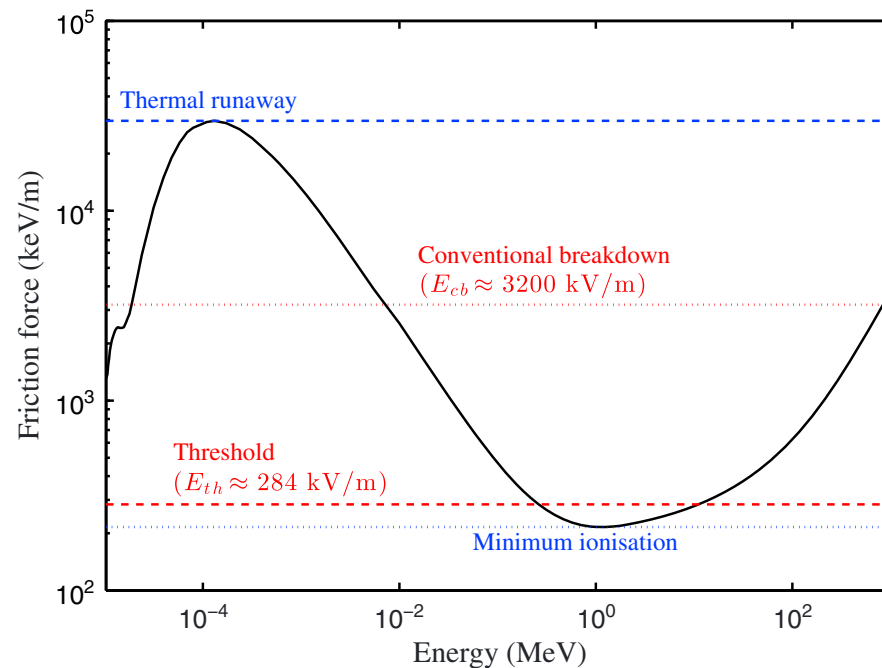
Figure 1. The friction force experienced by electrons in air at sea level with respect to their kinetic energy (solid black line). The dotted red line indicates the conventional breakdown field, E_{cb} = 3200 kV/m. The dashed red line shows the effective minimum threshold force experienced by runaway electrons and corresponds to E_{th} = 284 kV/m [Dwyer, 2003]. The dashed blue line shows the upper threshold for thermal runaway to occur, and the lower dotted blue line indicates the minimum ionization threshold. The data set was obtained from International Commission on Radiation Units and Measurements [1984].
